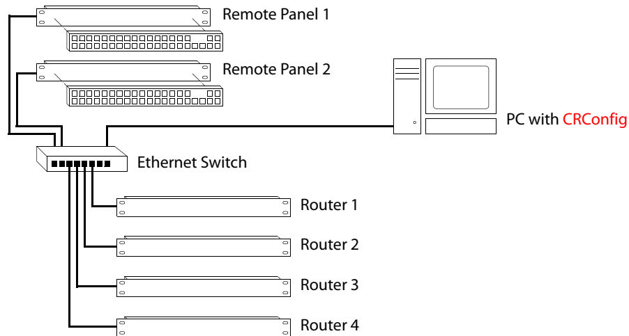
Fig. 3-2: Network of Routers
