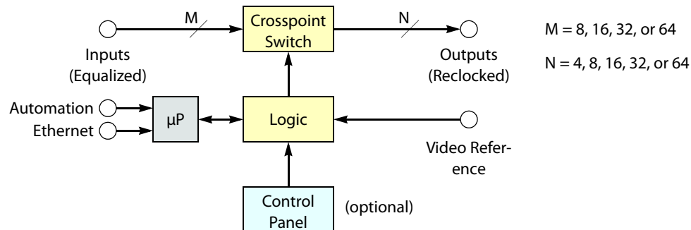
Fig. 2-18: Block Diagram of the Digital Video Router
