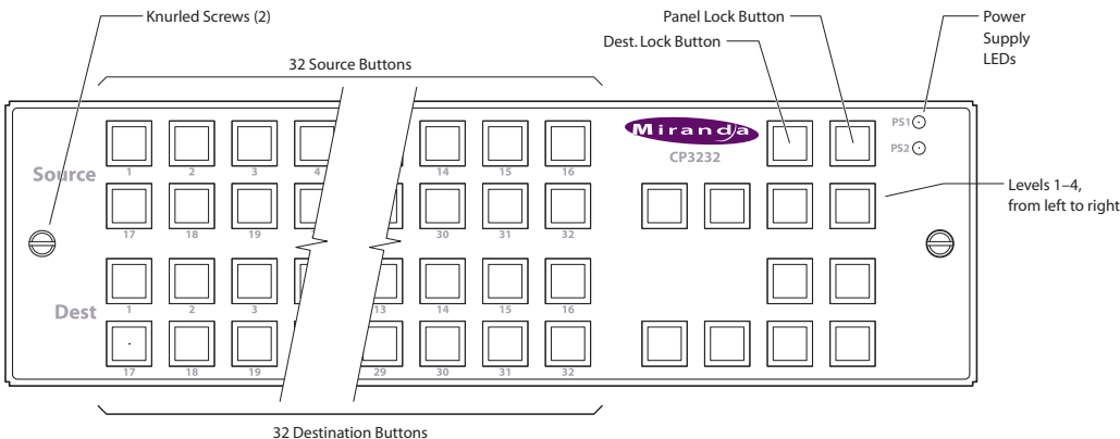
Fig. 2-71: Front View of the CP3232
