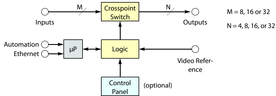
Fig. 2-22: Block Diagram of the Analog Video Router
