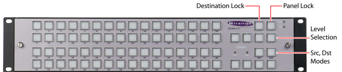
Fig. 2-28: Front view of the CP6464 Control Panel
