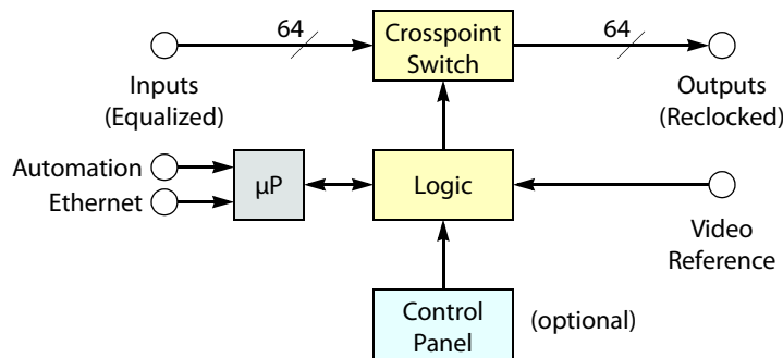
Fig. 2-21: Block Diagram of the CR Series
