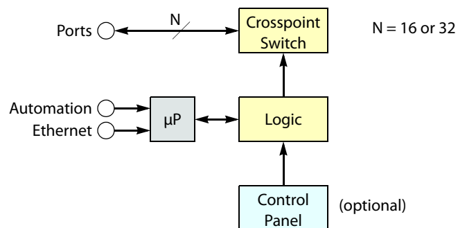
Fig. 2-25: Block Diagram of the Machine Control Router
