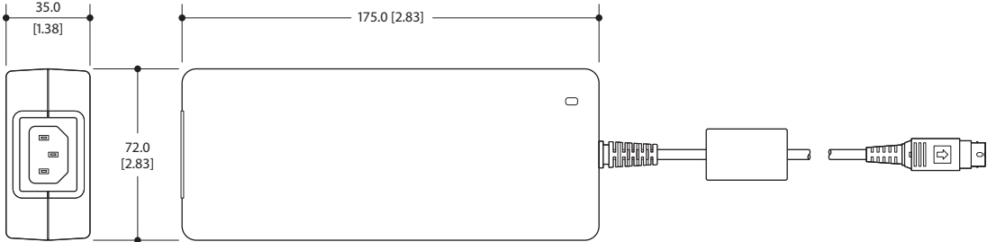
Fig. 12-2: Power Supply
