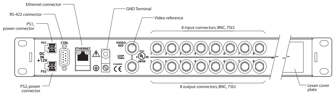
Fig. 2-38: Rear View, 8×8 Digital Router (3Gig, HD, SD, or AES)
