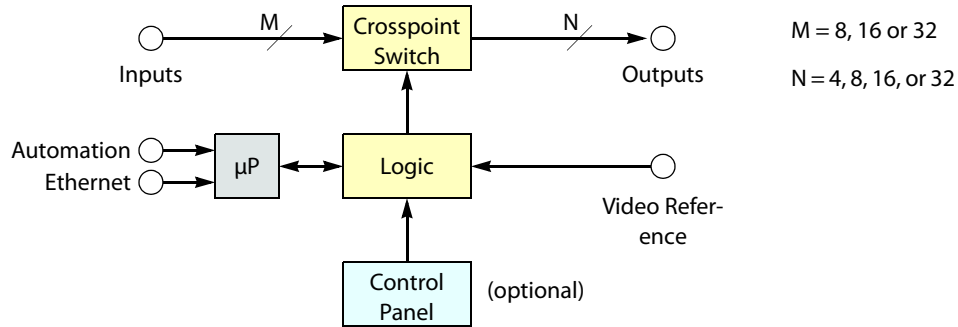
Fig. 2-24: Block Diagram of the Analog Audio Router
