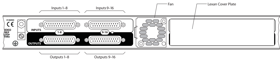
Fig. 2-46: Rear View, 8×8 Analog Audio Router
