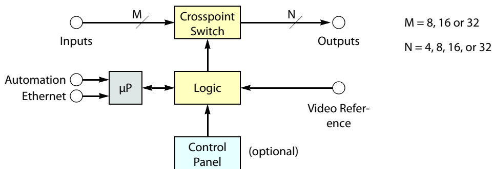
Fig. 2-23: Block Diagram of the AES Router
