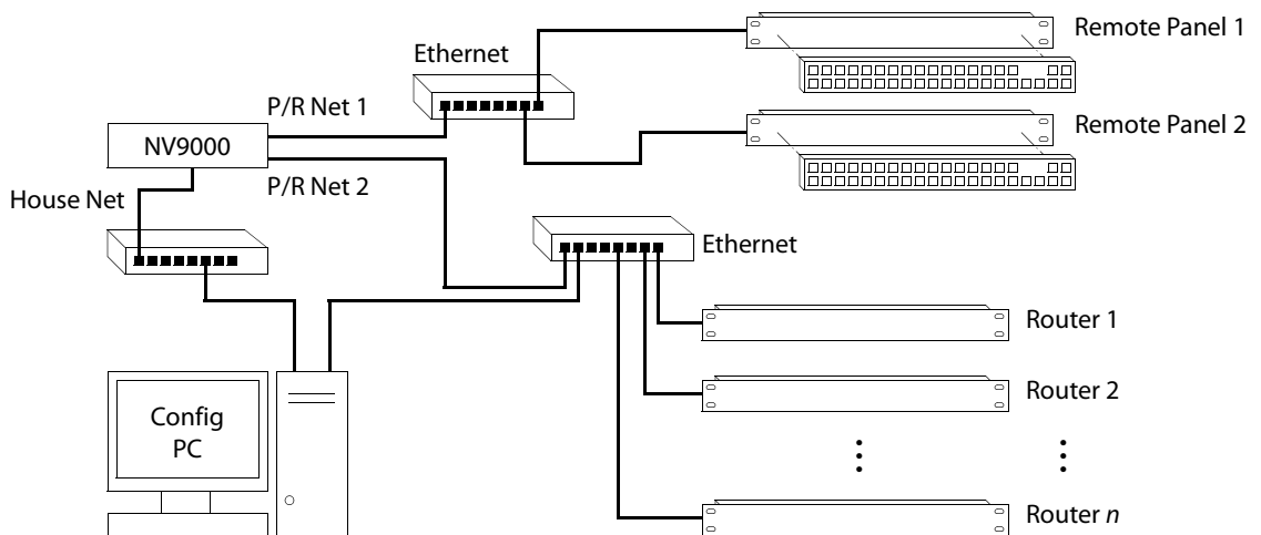
Fig. 2-2: NV9000 Network of Routers
