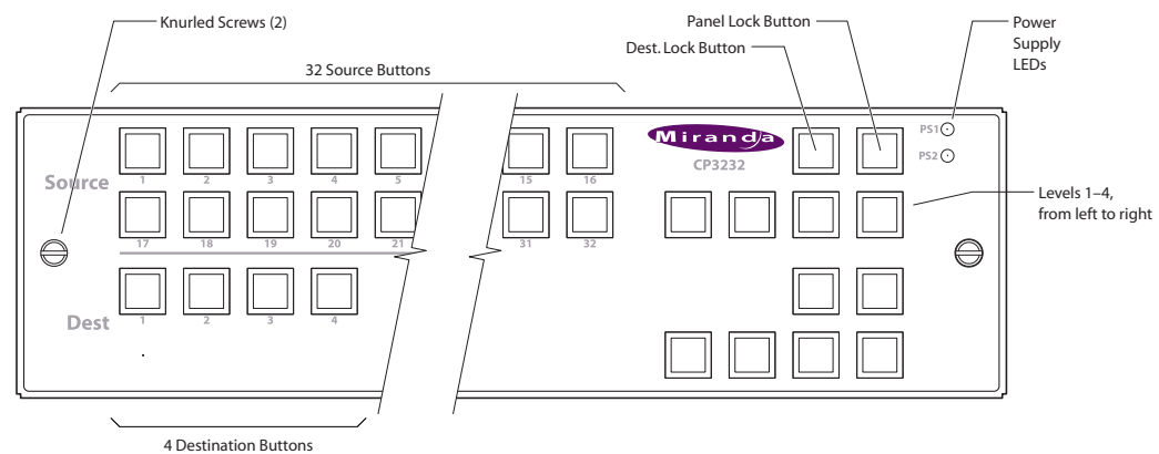
Fig. 2-73: Front View, CP3204
