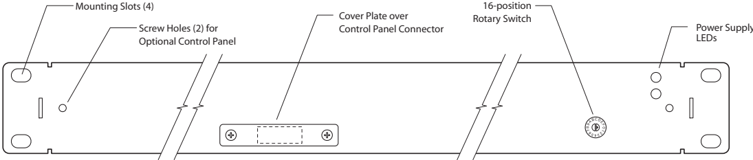
Fig. 2-74: Front View, RP16
