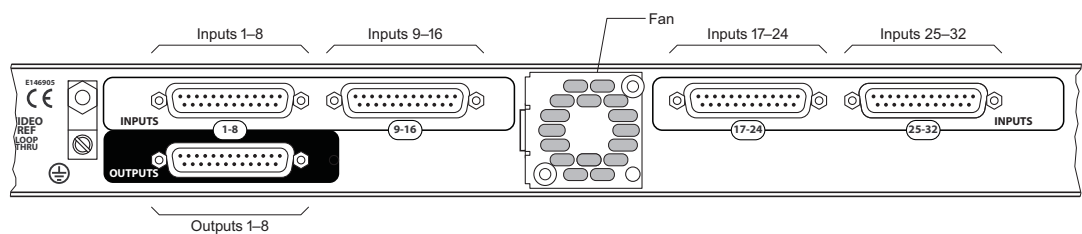
Fig. 2-44: Rear View, 16×4 Analog Audio Router
