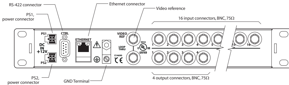
Fig. 2-36: Rear View, 16×4 Digital Router (3Gig, HD, SD, or AES)
