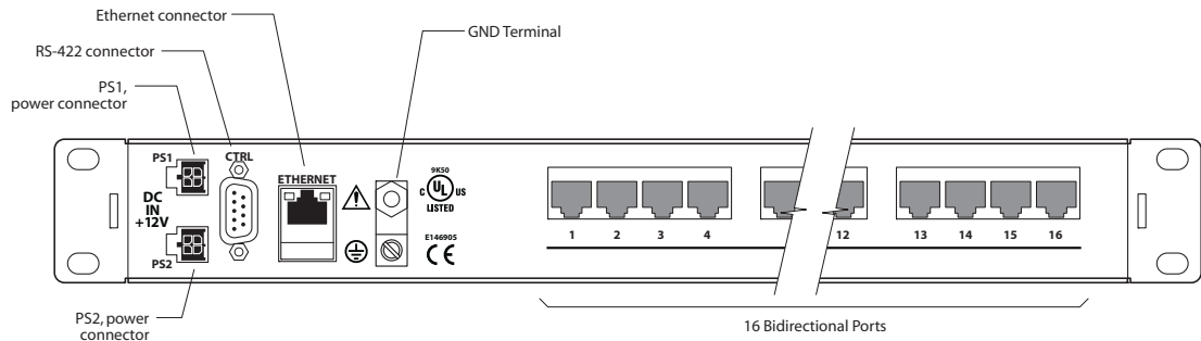
Fig. 2-47: Rear View, 16-Port Machine Control Router
