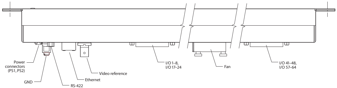
Fig. 2-60: Top View, 2RU Analog Audio Router
