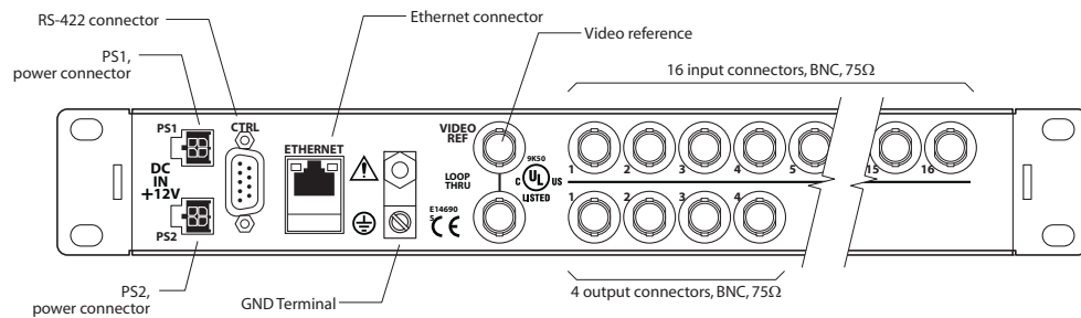
Fig. 2-41: Rear View, 16×4 Analog Video Router
