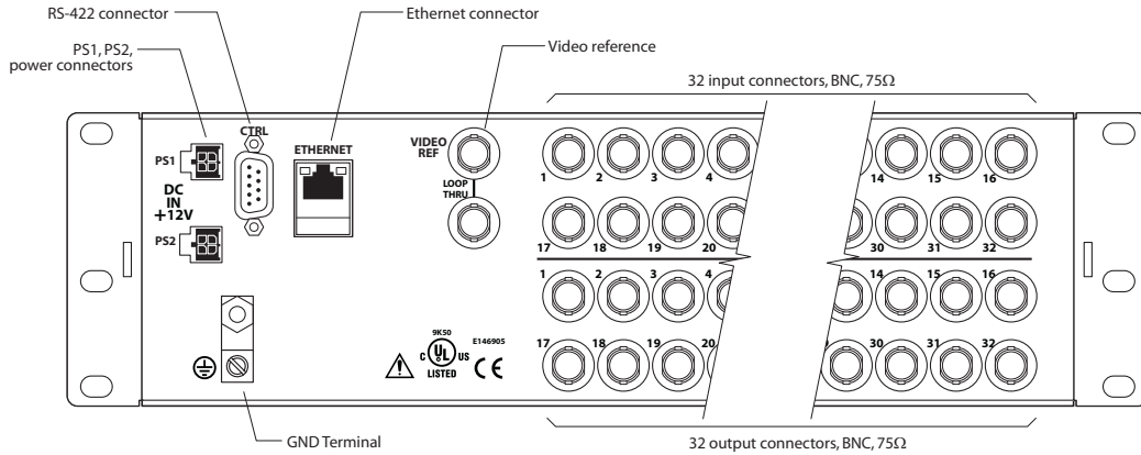
Fig. 2-53: Rear View, 32×32 3Gig, HD, SD, or AES Router
