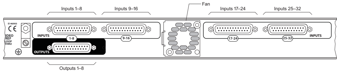
Fig. 2-44: Rear View, 16x4 Analog Audio Router
