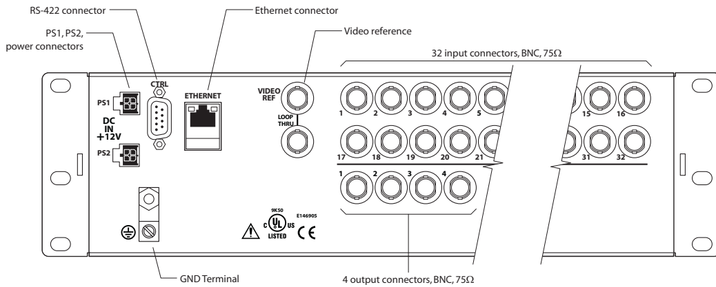
Fig. 2-54: Top View, 32×4 3Gig, HD, SD, AES, or Analog Video Router
