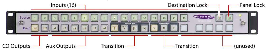
Fig. 2-27: Front view of the CP1602-CQX Control Panel
