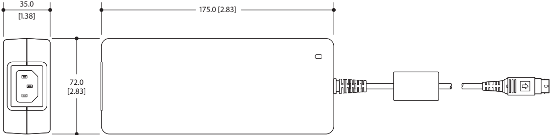
Fig. 12-2: Power Supply
