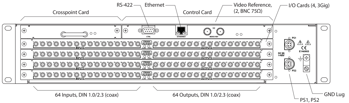
Fig. 2-51: Rear View, CR6400 Router (CR6464-3Gig Shown)
