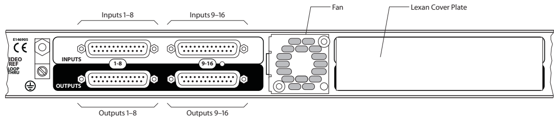
Fig. 2-46: Rear View, 8x8 Analog Audio Router
