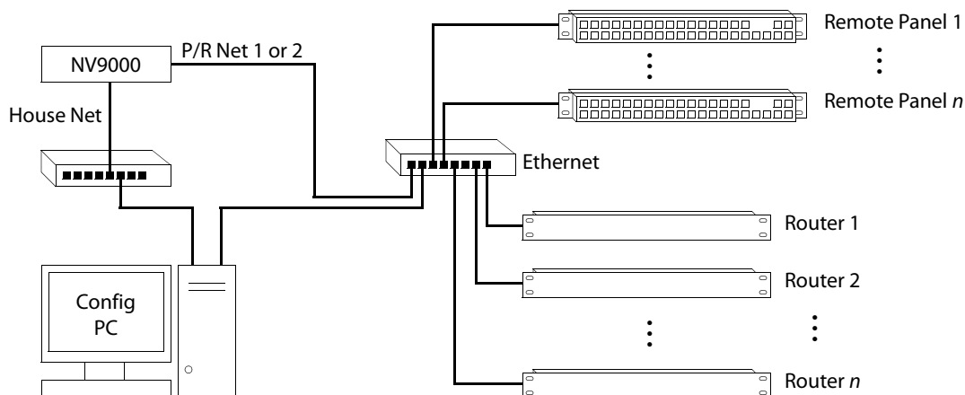
Fig. 3-5: NV9000 Network of Routers
