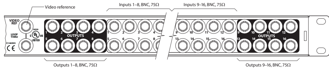
Fig. 2-40: Rear View, 16×16 Analog Video Router
