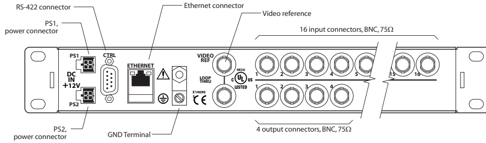
Fig. 2-36: Rear View, 16x4 Digital Router (3Gig, HD, SD, or AES)
