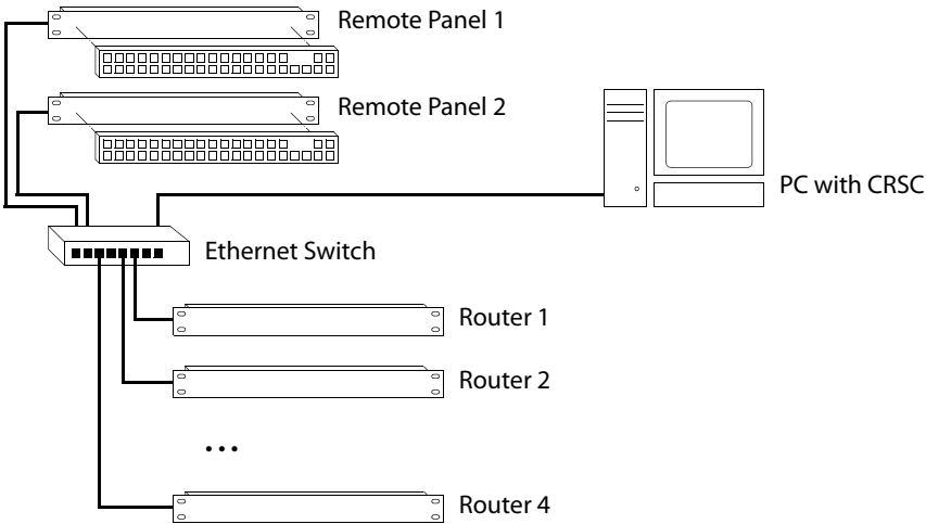
Fig. 3-3: Network of Routers
