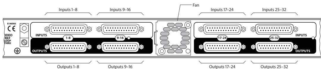
Fig. 2-43: Rear View, 16×16 Analog Audio Router
