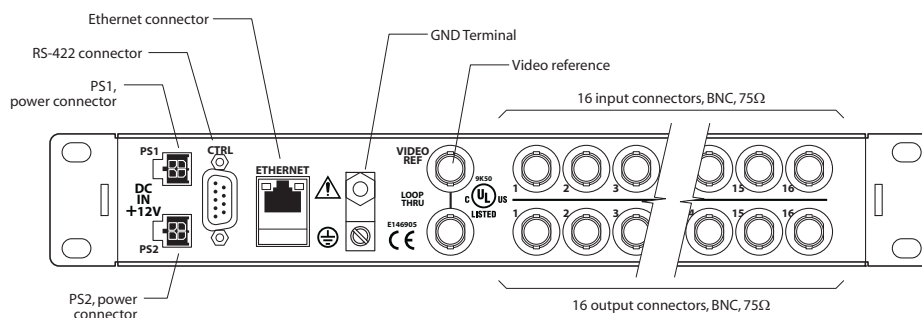
Fig. 2-35: Rear View, 1RU Router (3Gig, HD, SD, or AES)
