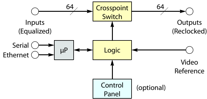
Fig. 2-21: Block Diagram of the CR Series
