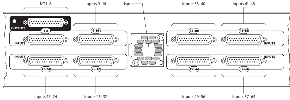
Fig. 2-59: Rear View, 32x4 Analog Audio Router
