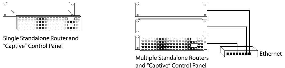
Fig. 2-4: CR6400 Usage
