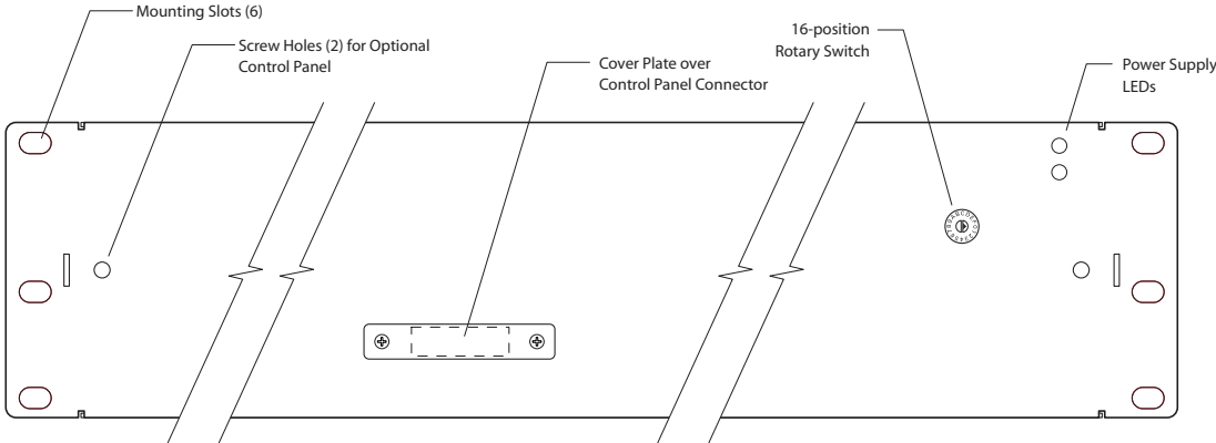
Fig. 2-77: Front View, RP32
