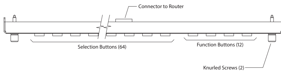
Fig. 2-70: Top View of the CP6464
