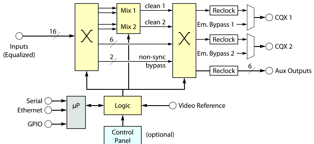
Fig. 2-19: Block Diagram of the CQX Digital Video Router
