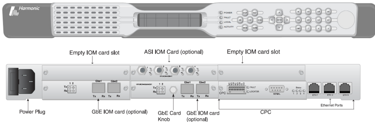
Prostream 1000 front and back panels
