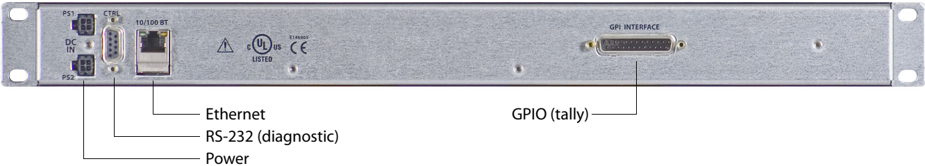
Fig. 2-2: NV9641 rear
