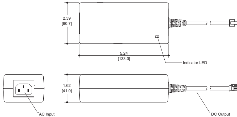
Fig. 7-1: The power output has Molex 4-pin plug. See Power Cord Retention on page 86.
